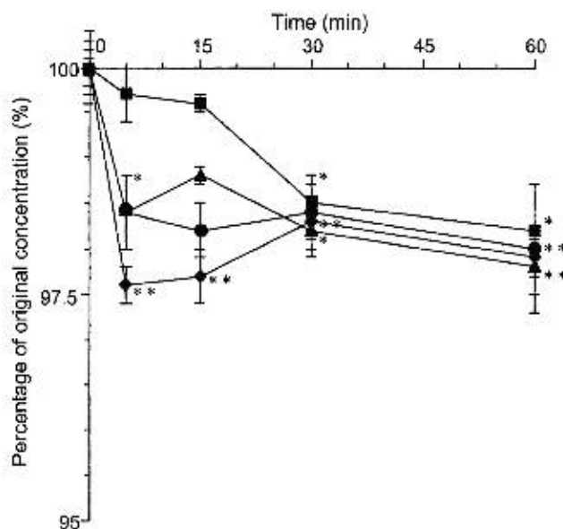
Figure 4. Concentration changes of local anesthetics flowing out of infusion balloons injected with their solutions of pH 6.0. The sample solutions (1.0 mM each) were injected into the balloons of 100-mL volume, and the effluents were analyzed over time by high-performance liquid chromatography: lidocaine (●), bupivacaine (◆), ropivacaine (▲), and mepivacaine (■). Data are mean \pm SE ( n = 4 ). * P < 0.05 and ** P < 0.01 ; significantly different from initial concentration (0 min).
